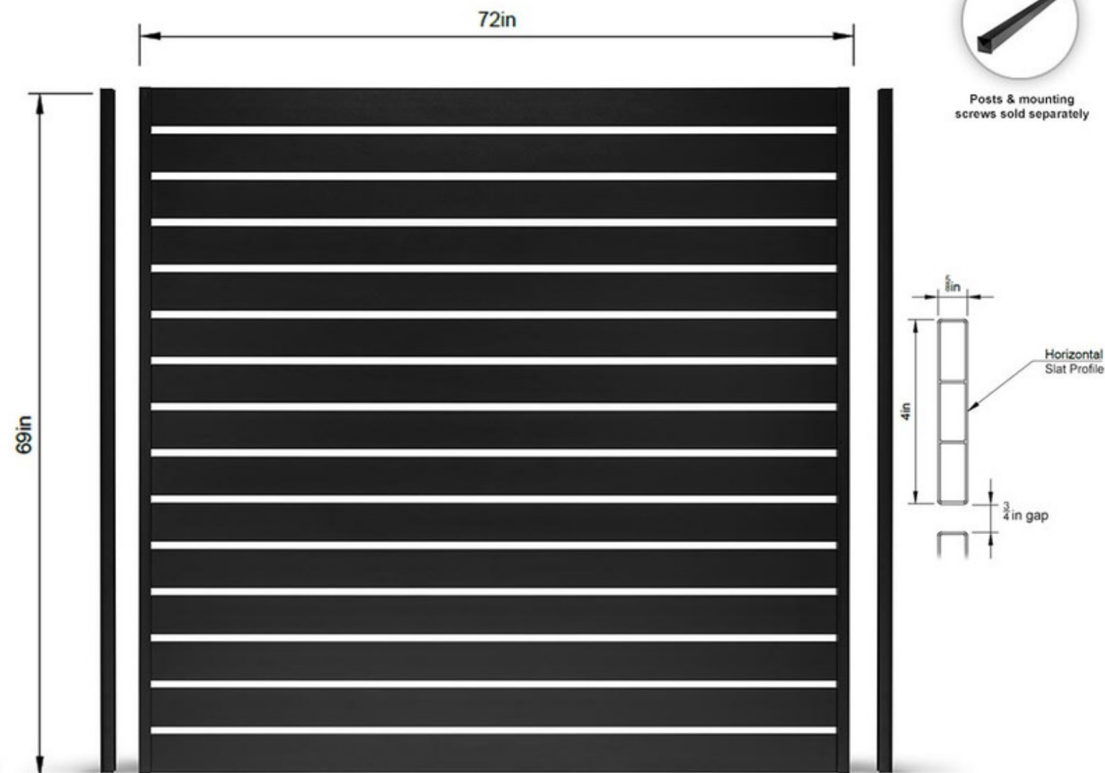
SKU 1008 - Preassembled Screen Panel
