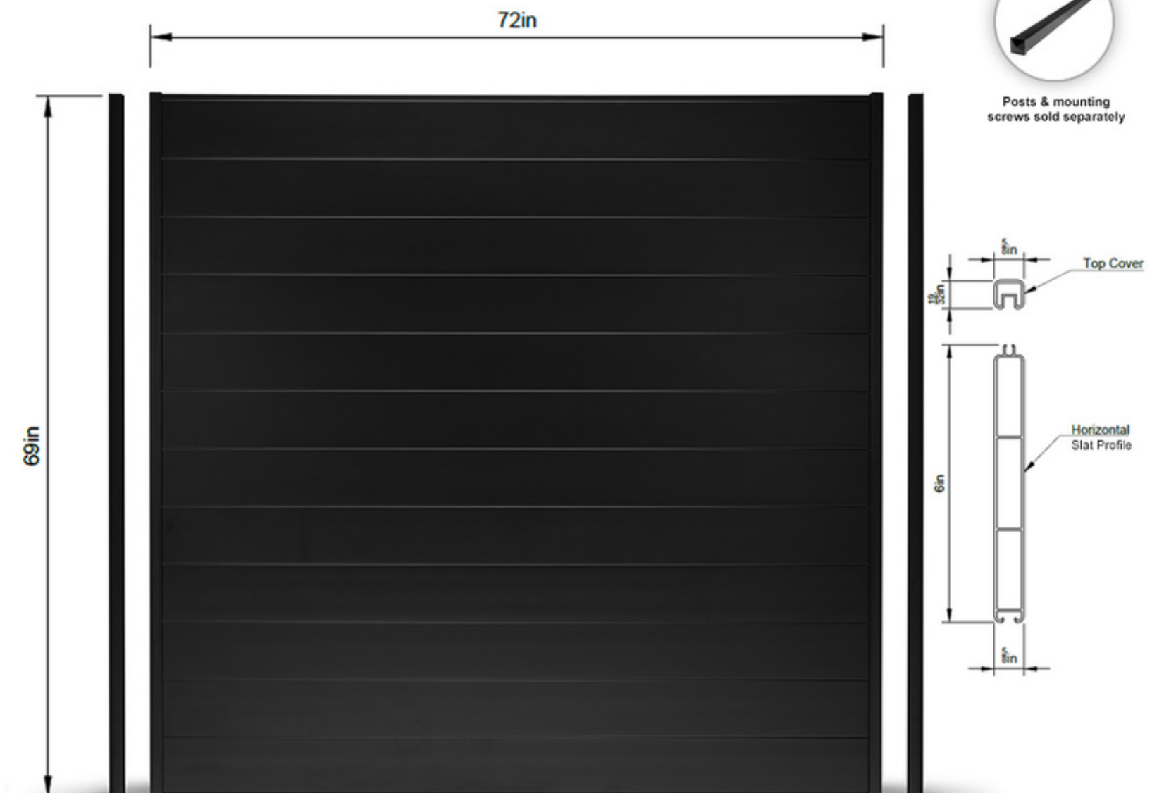
SKU 1006 - Preassembled Privacy Panel
